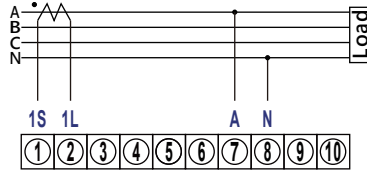
3 Phase 4 Wire
