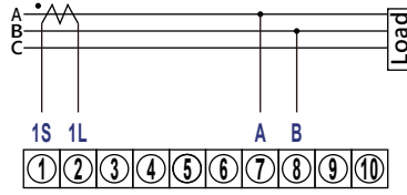
3 Phase 3 Wire
