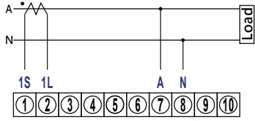
1 Phase 2 Wire
