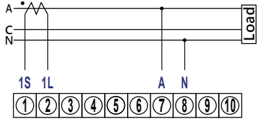
1 Phase 3 Wire
