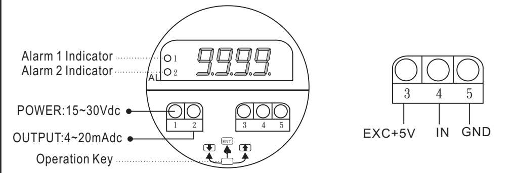
Wiring connection
