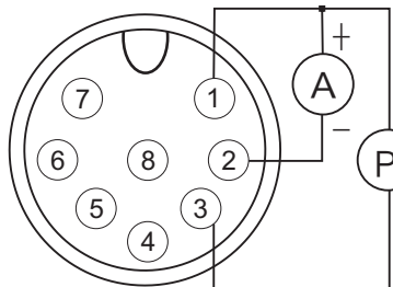
Wiring connection
